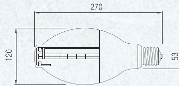
550/750/1,000W (U-TYPE)
