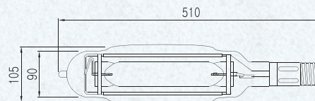
MQ4000H2-C
