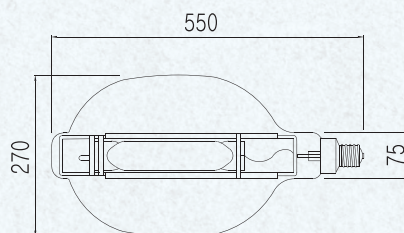
MF3000H2-C
