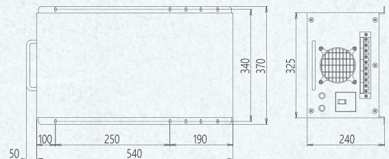
KSL-100F MH-100F
