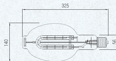
2,000/3,000W (U-TYPE)
