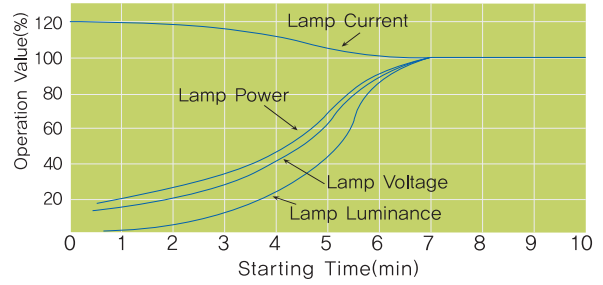
Starting characteristics
