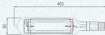
MQ2000H2-C
